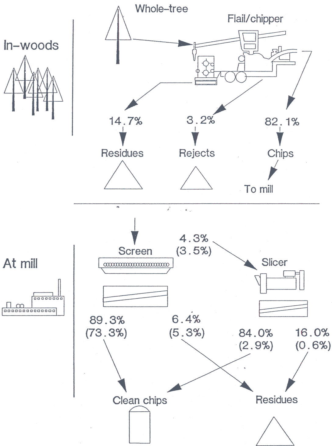
Figure 2. Product flow--in-woods flail/chip option (value in parentheses represents percentage of whole tree).
