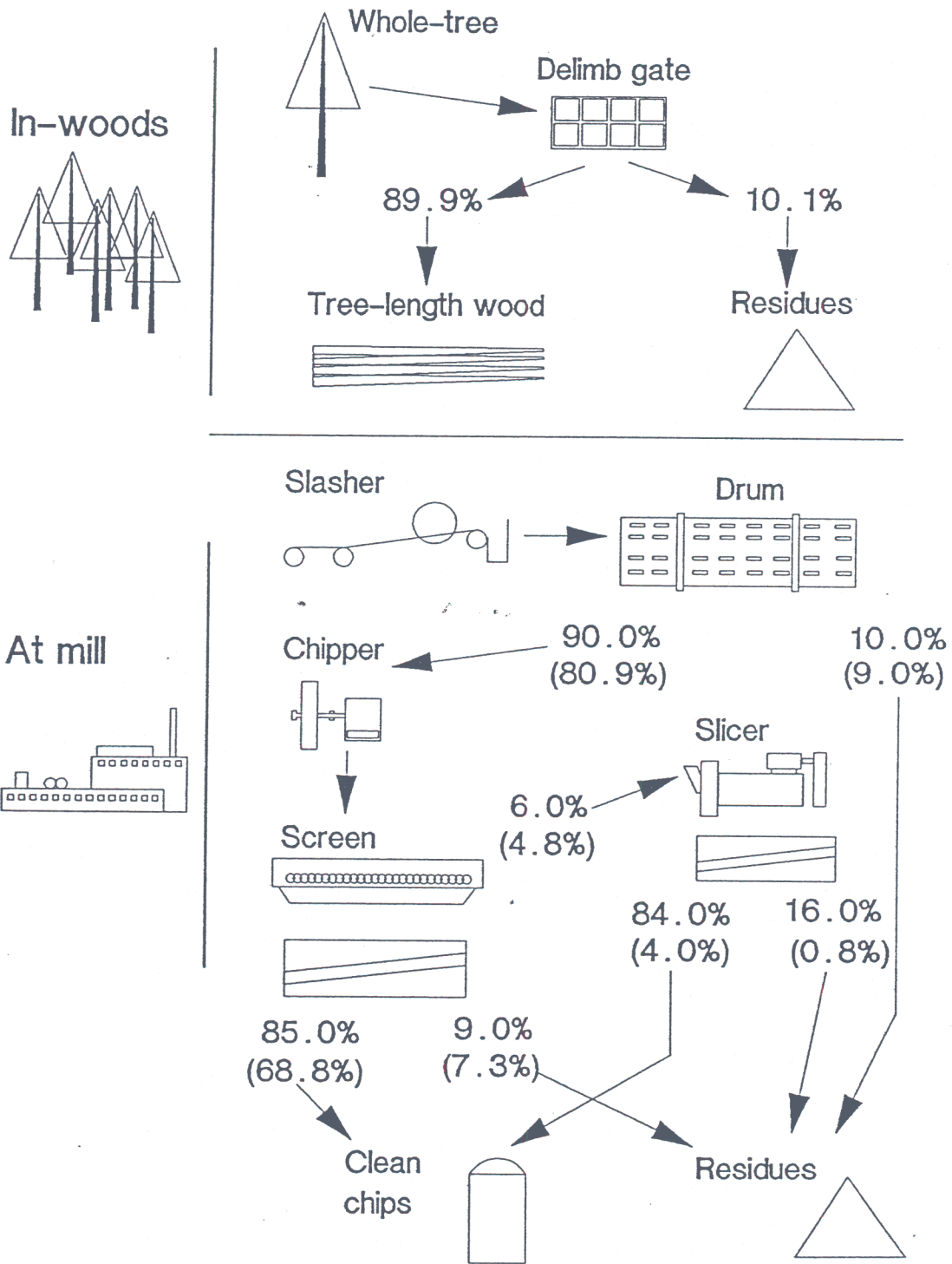
Figure 1. Product flow--tree-length option (value in parentheses represents percentage of whole tree).
