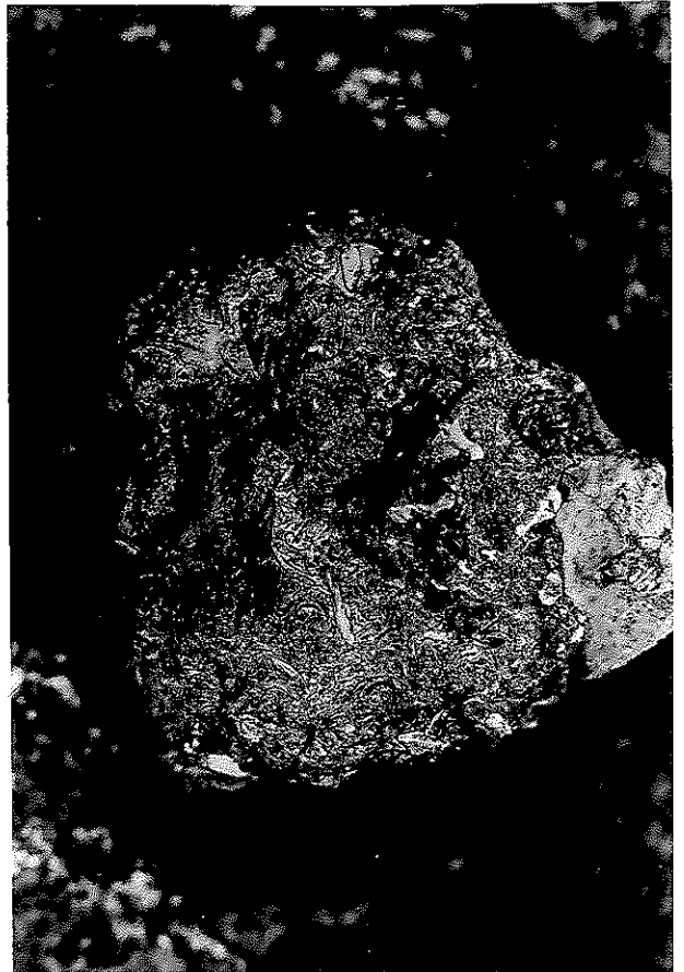
Limestone parent material underlying Grand Prairie soils
